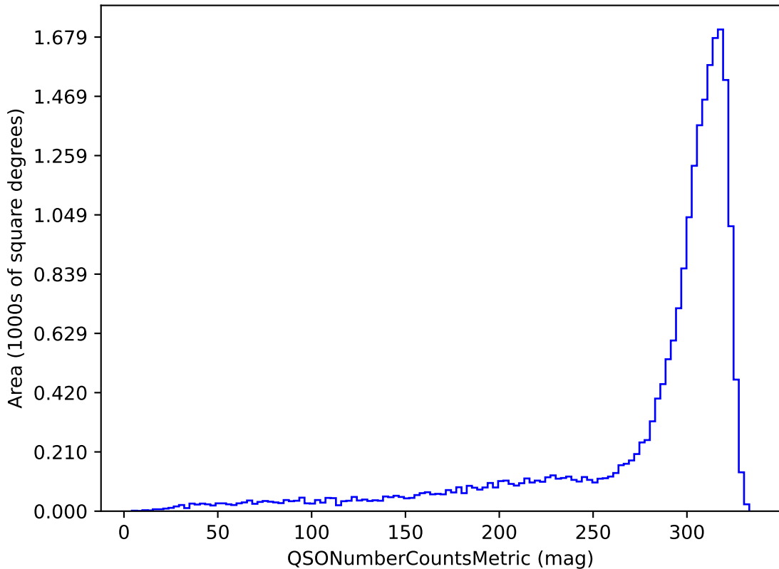
ddf_loaded_fl8_v3.4_10yrs u band and non-DD: QSONumberCountsMetric
