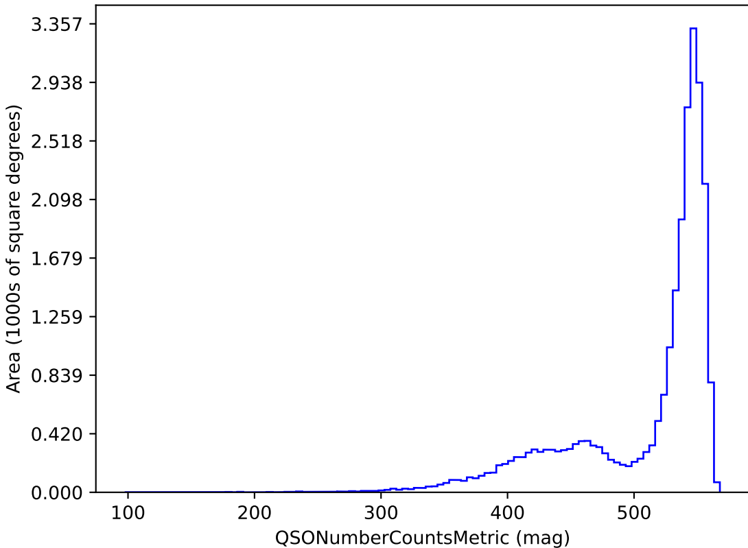
ddf_loaded_fl8_v3.4_10yrs i band and non-DD: QSONumberCountsMetric
