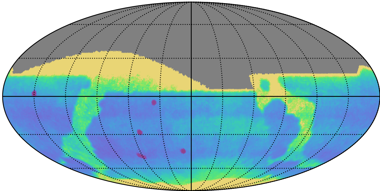
ddf_loaded_fl8_v3.4_10yrs : Proper Motion Uncert @ 24.0
