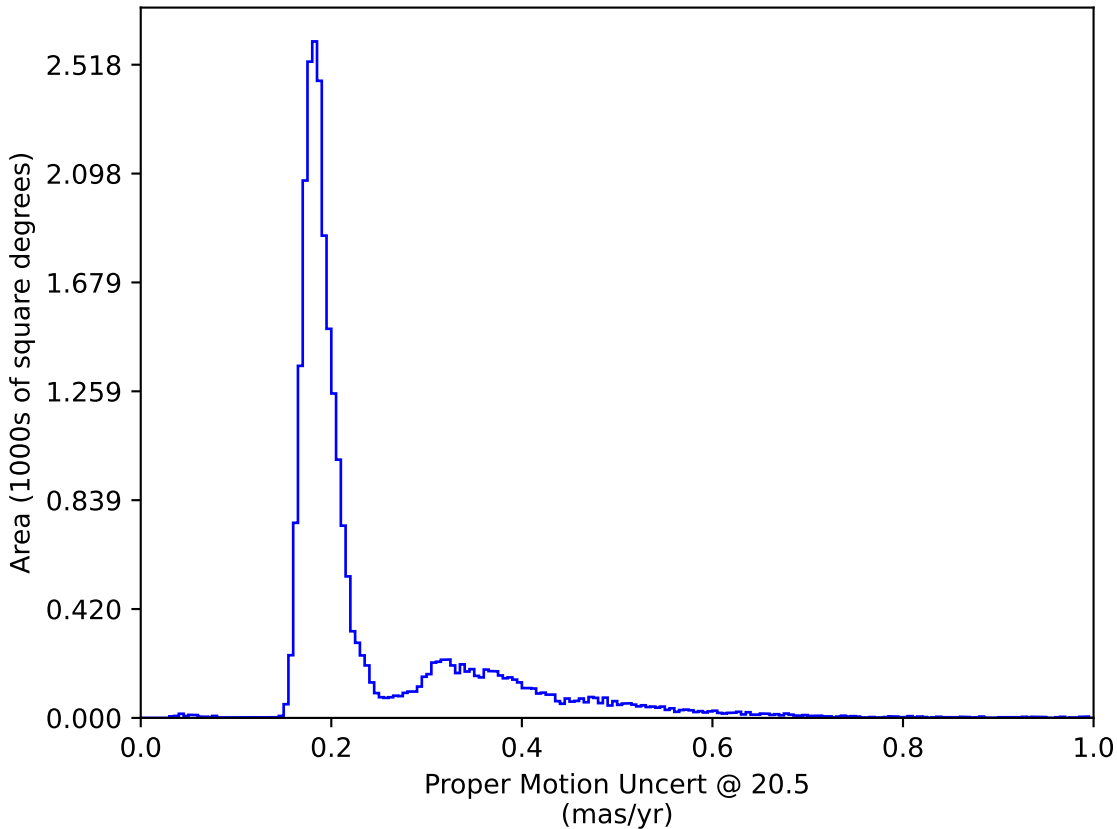
ddf_loaded_fl8_v3.4_10yrs : Proper Motion Uncert @ 20.5
