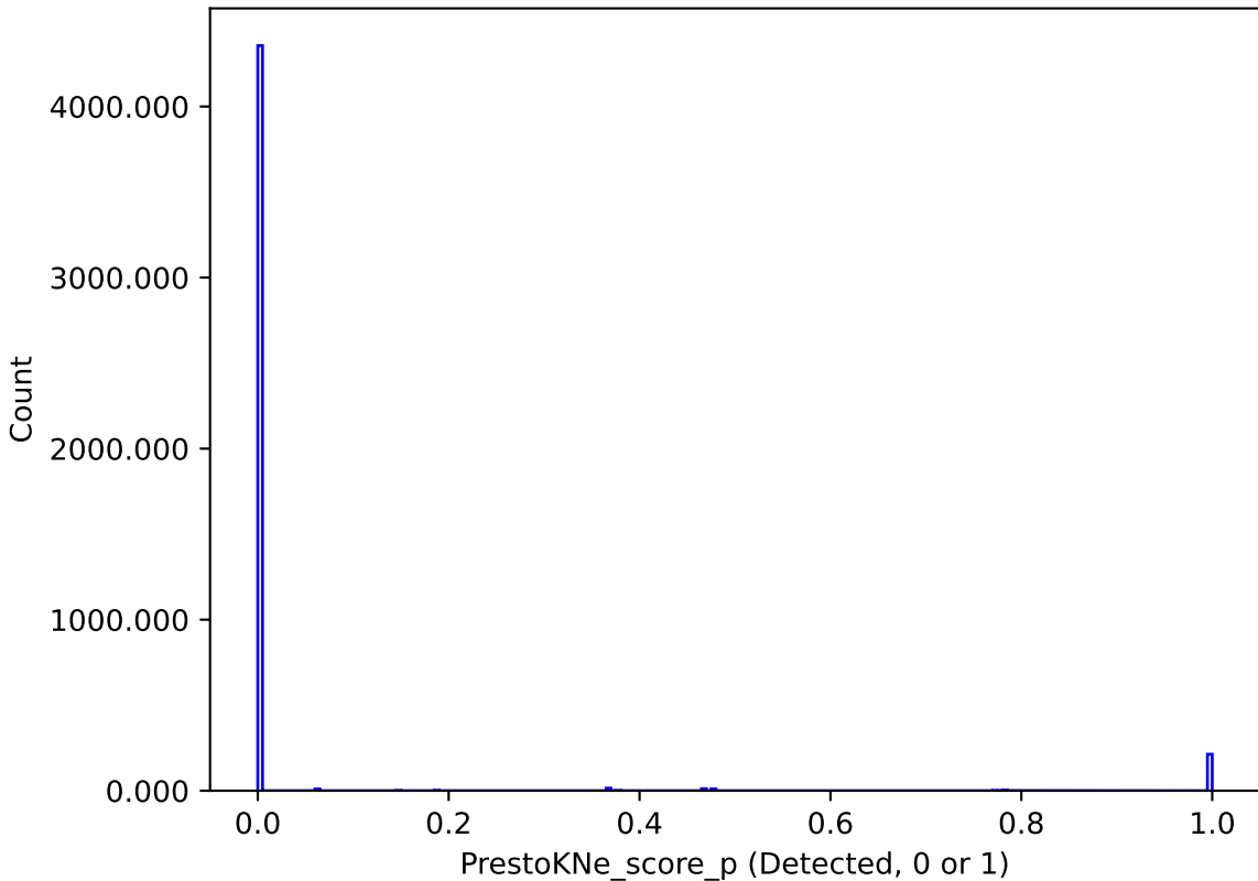
ddf_loaded_fl8_v3.4_10yrs : PrestoKNe_score_p
