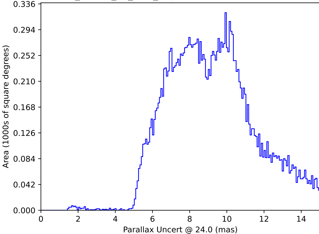
ddf_loaded_fl8_v3.4_10yrs : Parallax Uncert @ 24.0
