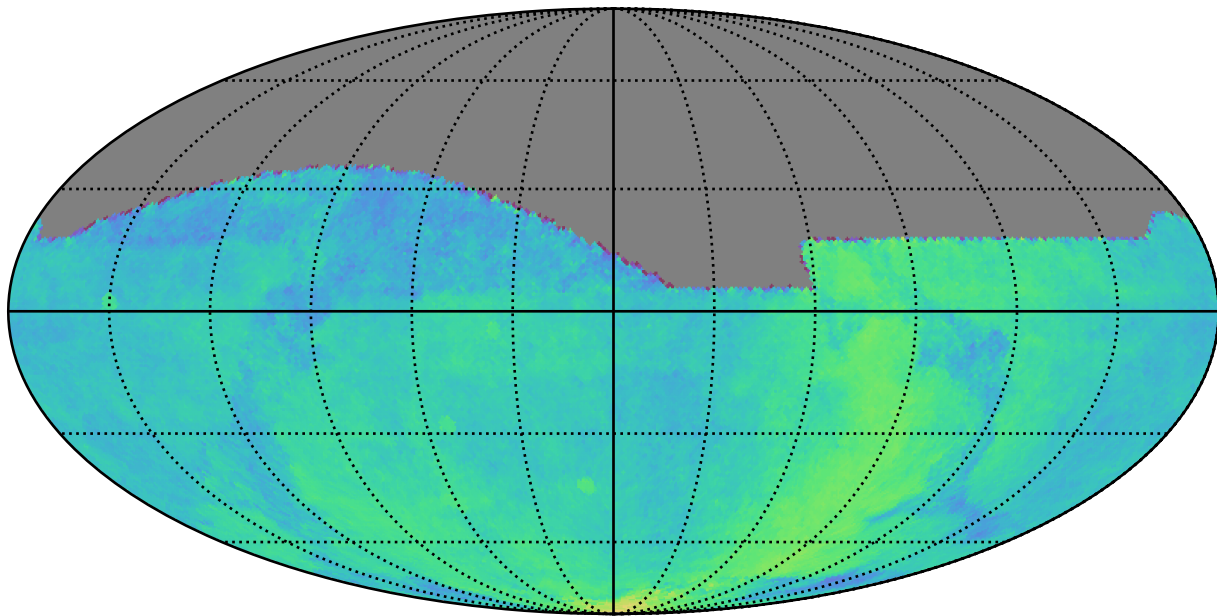
ddf_loaded_fl8_v3.4_10yrs : Parallax Coverage @ 24.0
