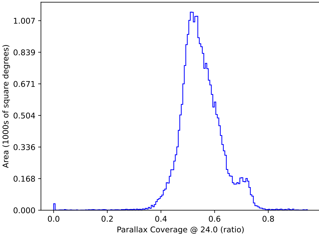
ddf_loaded_fl8_v3.4_10yrs : Parallax Coverage @ 24.0
