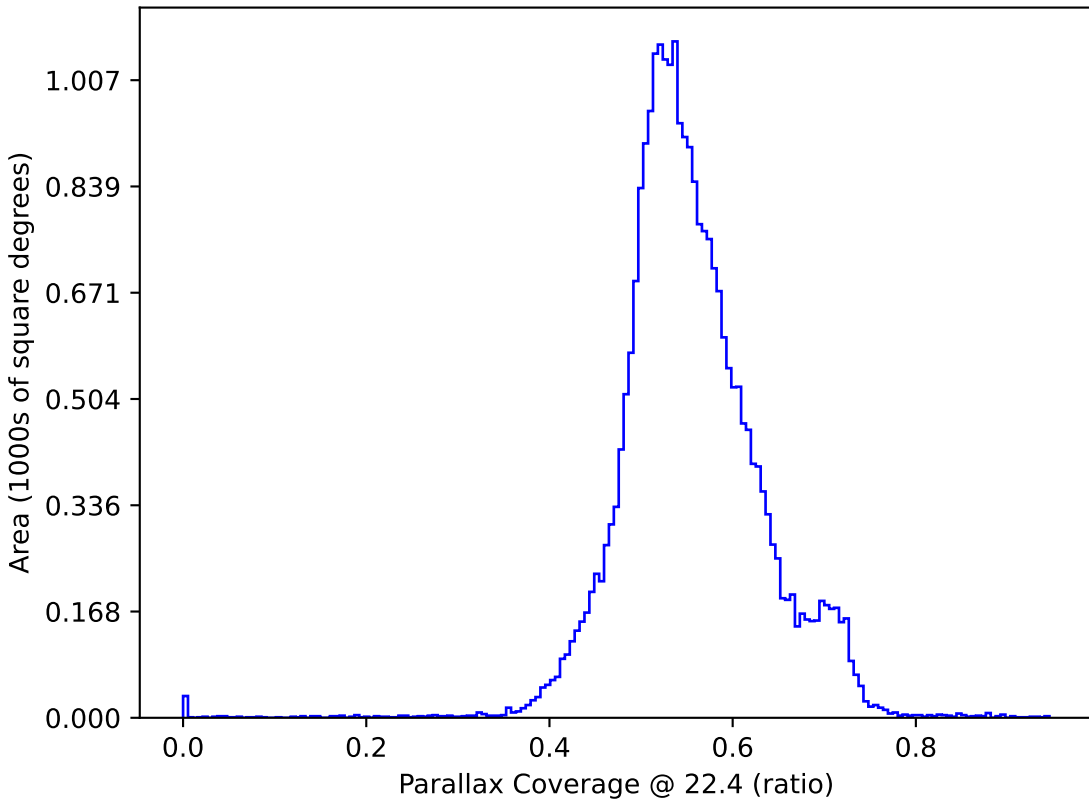
ddf_loaded_fl8_v3.4_10yrs : Parallax Coverage @ 22.4
