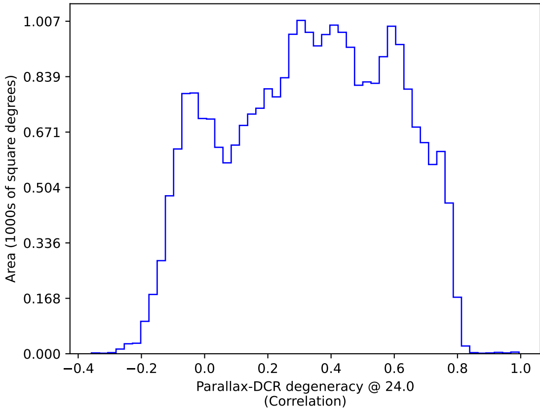
ddf_loaded_fl8_v3.4_10yrs : Parallax-DCR degeneracy @ 24.0
