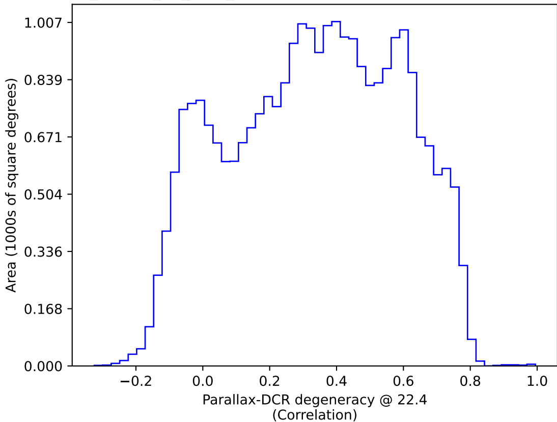
ddf_loaded_fl8_v3.4_10yrs : Parallax-DCR degeneracy @ 22.4
