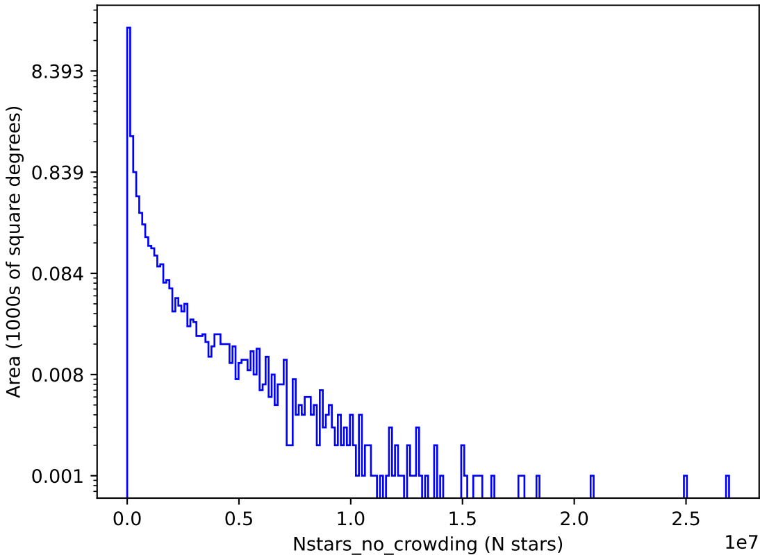
ddf_loaded_fl8_v3.4_10yrs z: Nstars_no_crowding
