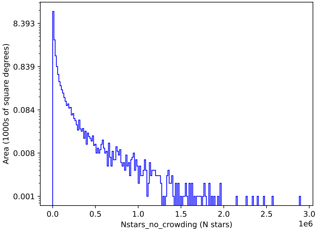
ddf_loaded_fl8_v3.4_10yrs u: Nstars_no_crowding
