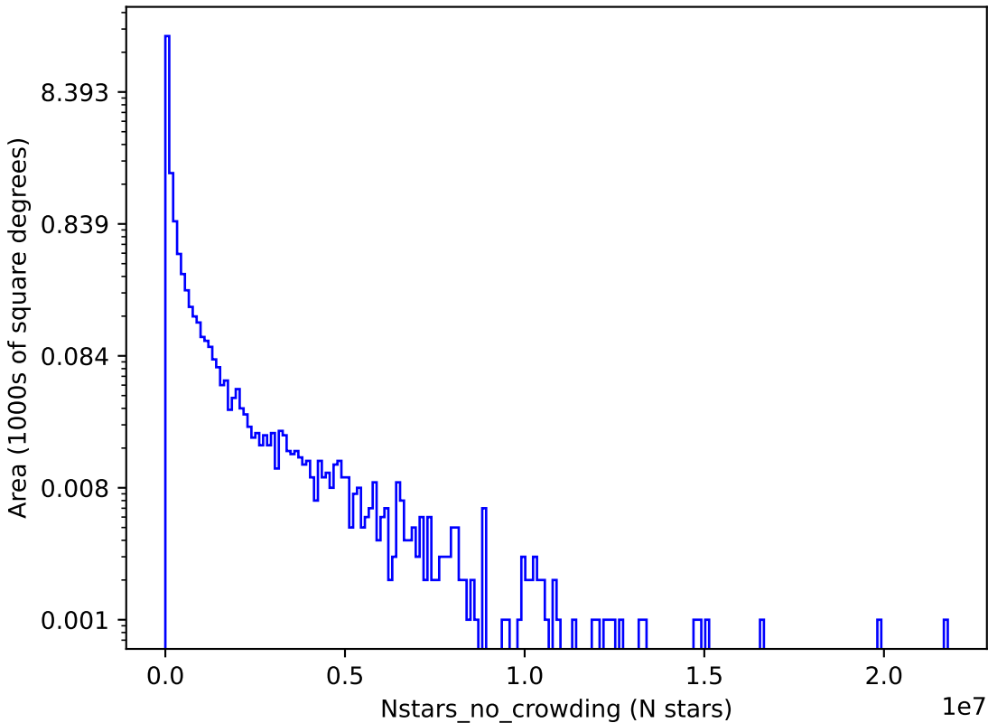
ddf_loaded_fl8_v3.4_10yrs r: Nstars_no_crowding
