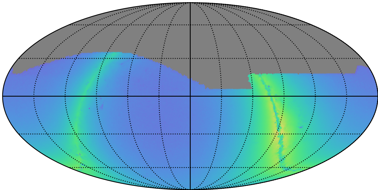
ddf_loaded_fl8_v3.4_10yrs i: Nstars_no_crowding
