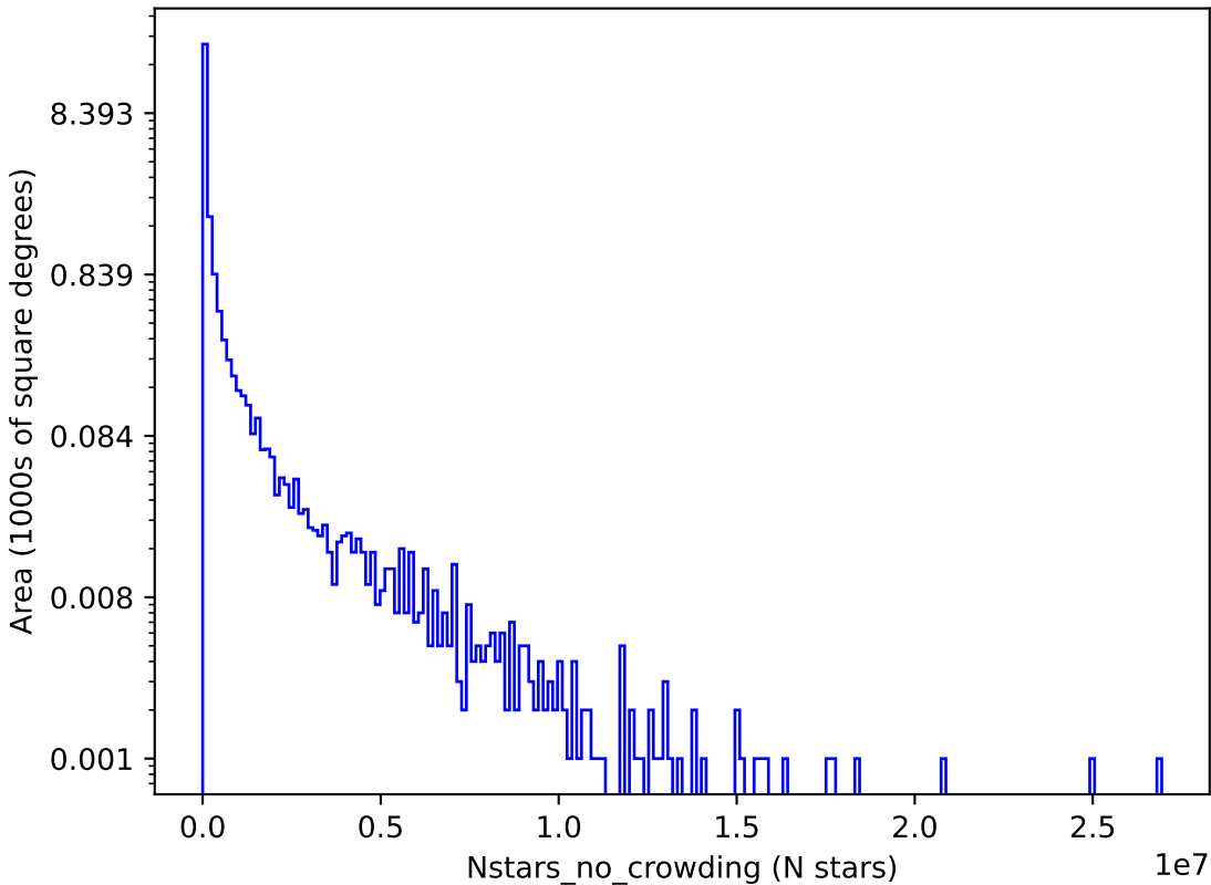
ddf_loaded_fl8_v3.4_10yrs i: Nstars_no_crowding
