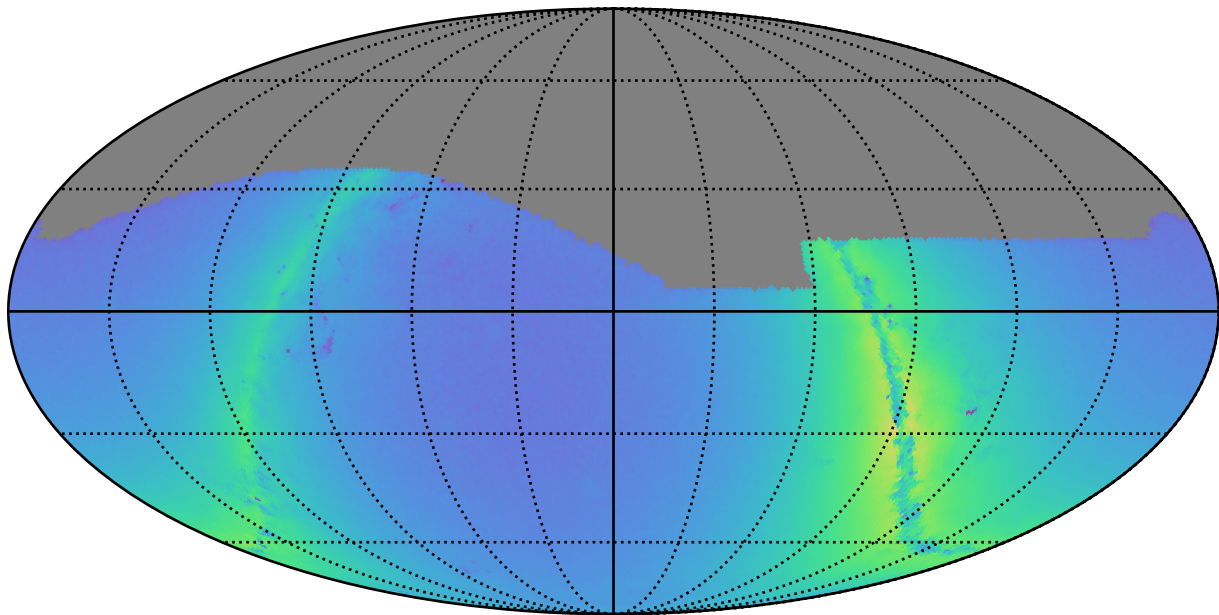
ddf_loaded_fl8_v3.4_10yrs g: Nstars_no_crowding
