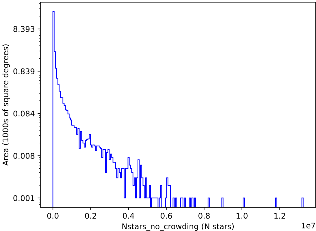
ddf_loaded_fl8_v3.4_10yrs g: Nstars_no_crowding
