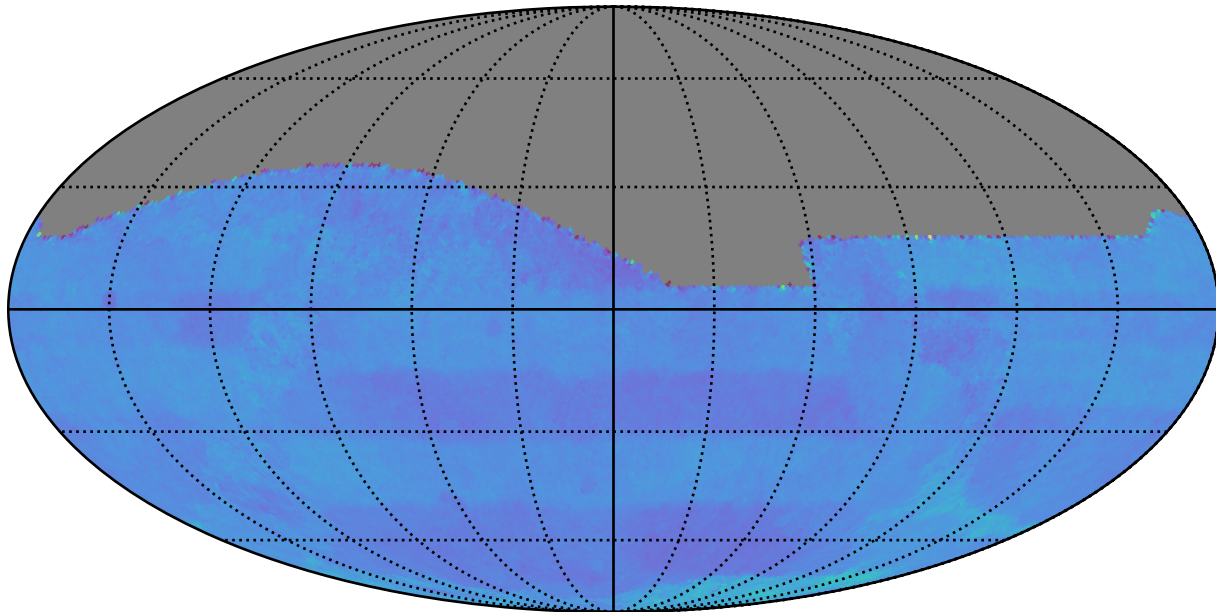
ddf_loaded_fl8_v3.4_10yrs : Normalized Proper Motion Uncert @ 24.0
