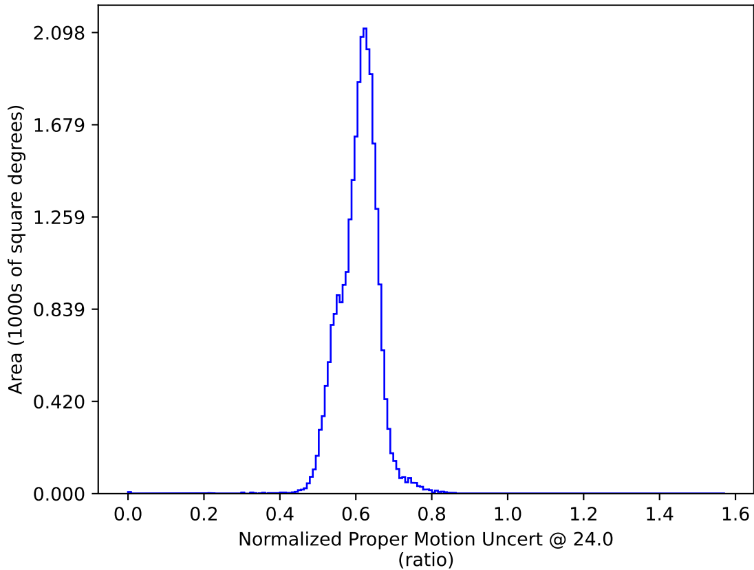
ddf_loaded_fl8_v3.4_10yrs : Normalized Proper Motion Uncert @ 24.0
