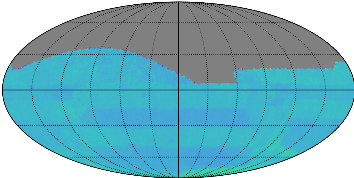
ddf_loaded_fl8_v3.4_10yrs : Normalized Proper Motion Uncert @ 20.5
