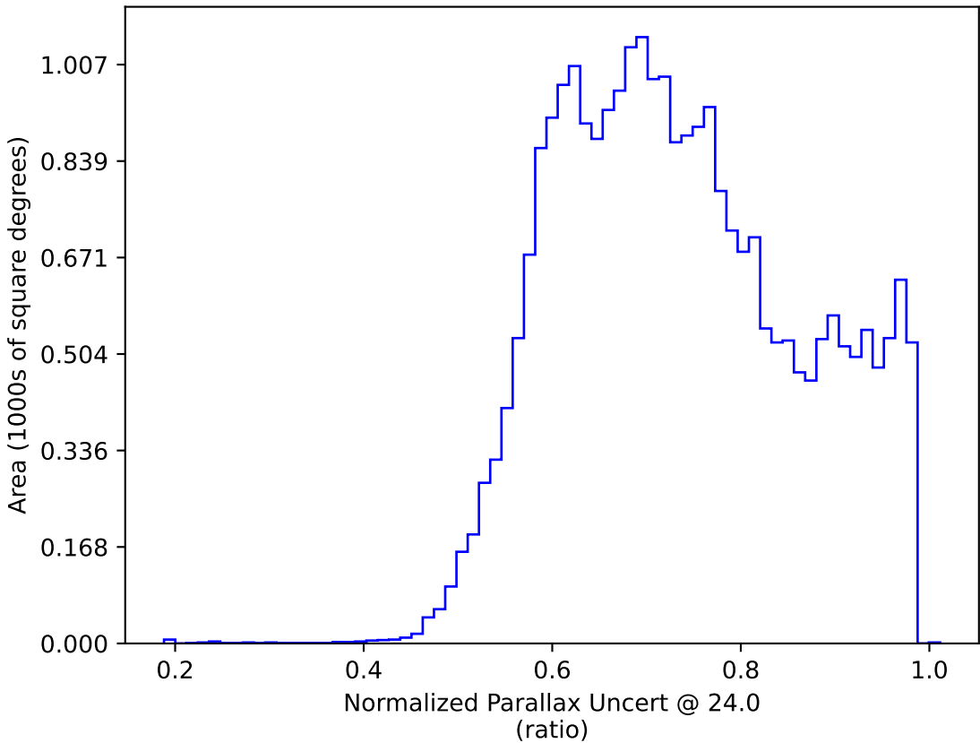
ddf_loaded_fl8_v3.4_10yrs : Normalized Parallax Uncert @ 24.0
