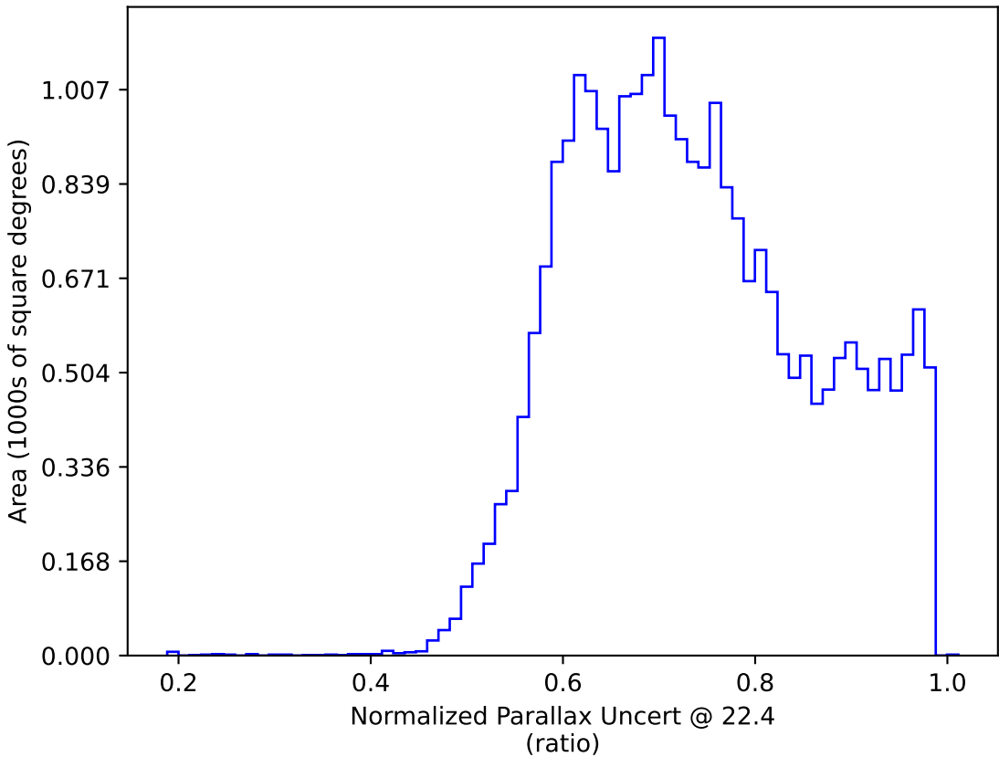
ddf_loaded_fl8_v3.4_10yrs : Normalized Parallax Uncert @ 22.4
