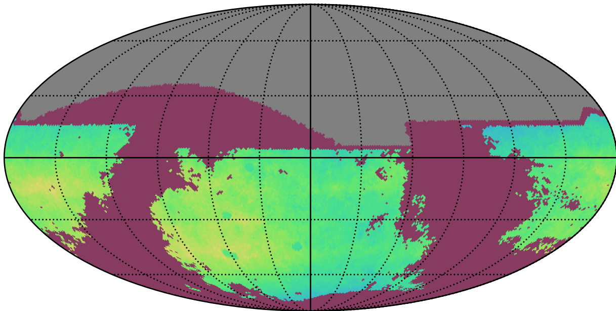
ddf_loaded_fl8_v3.4_10yrs i: NgalScale
