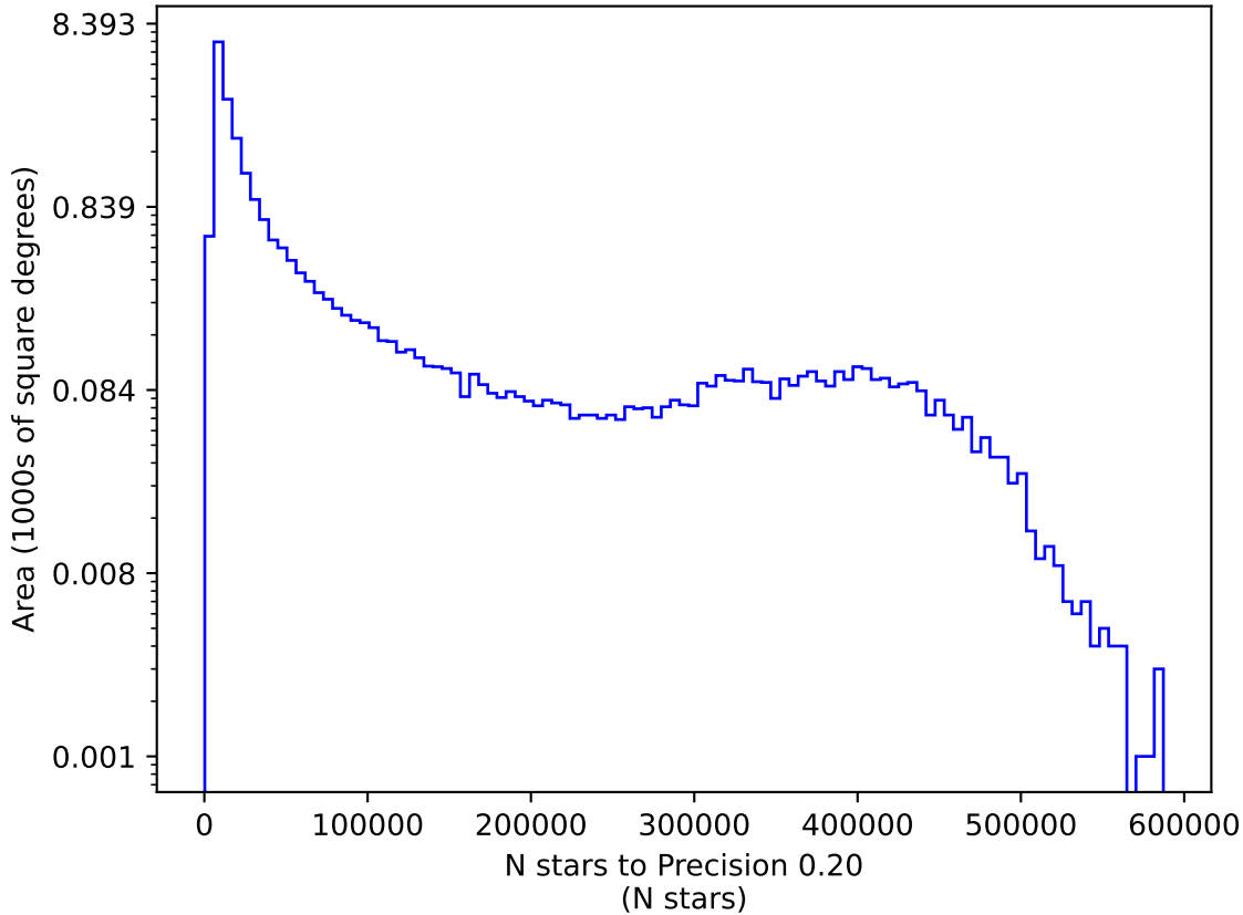
ddf_loaded_fl8_v3.4_10yrs y: N stars to Precision 0.20
