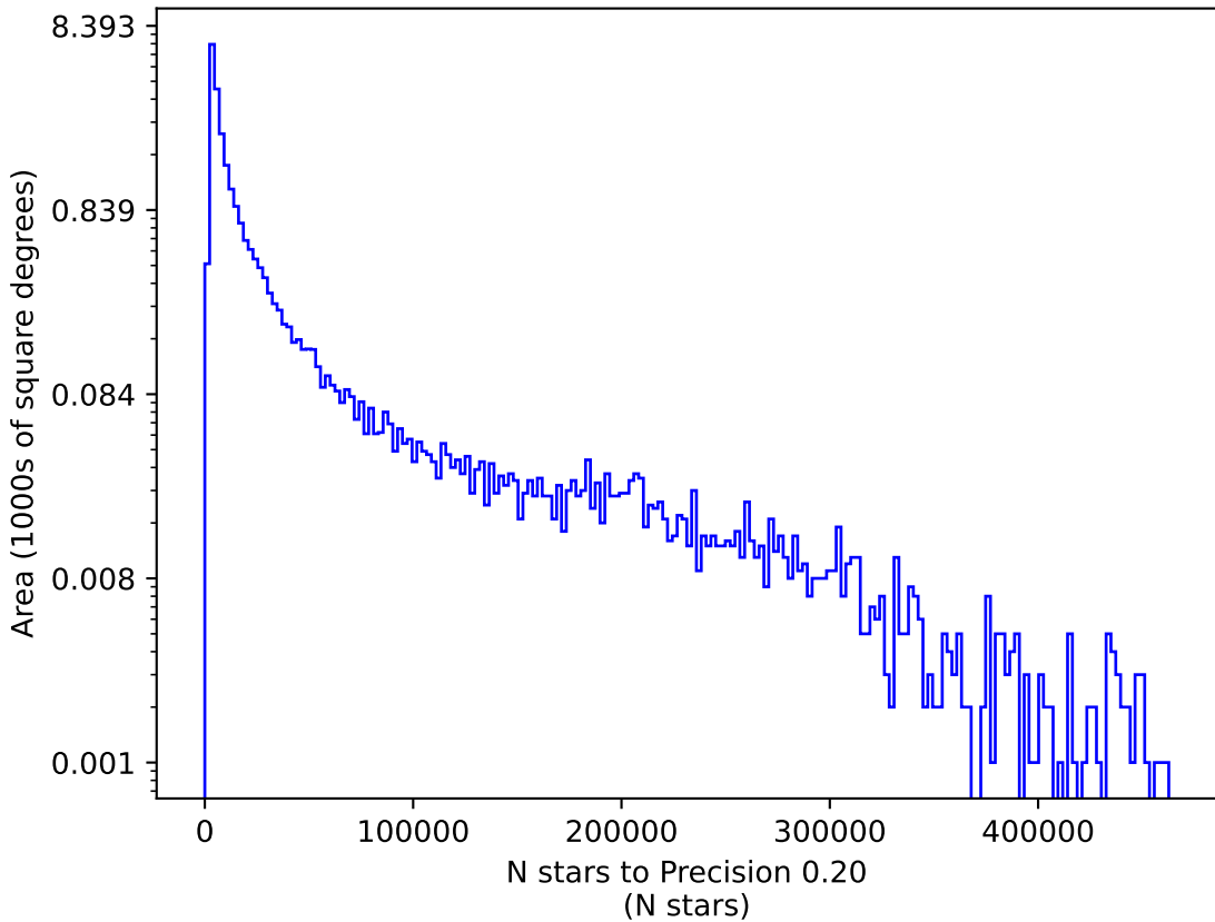
ddf_loaded_fl8_v3.4_10yrs u: N stars to Precision 0.20
