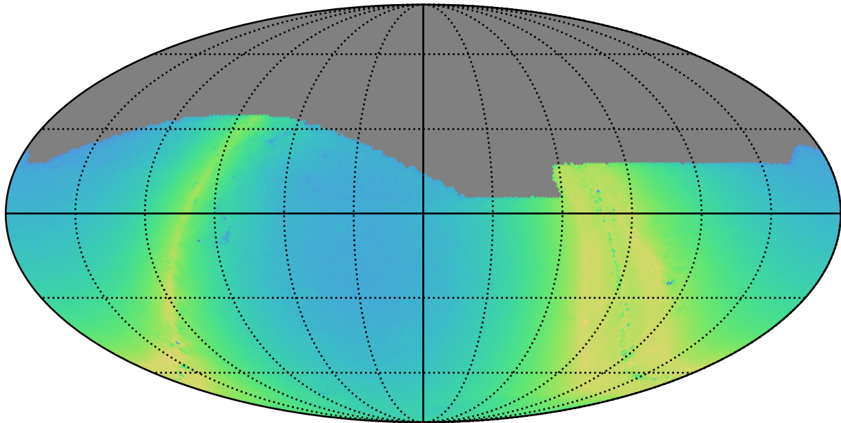
ddf_loaded_fl8_v3.4_10yrs r: N stars to Precision 0.20
