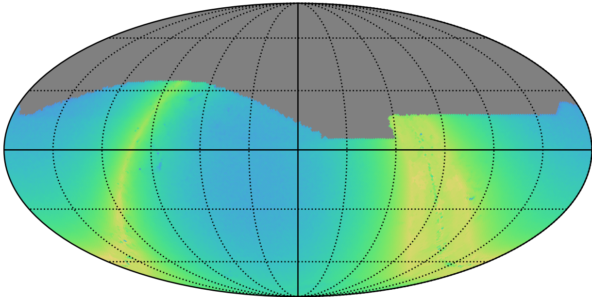
ddf_loaded_fl8_v3.4_10yrs i: N stars to Precision 0.20
