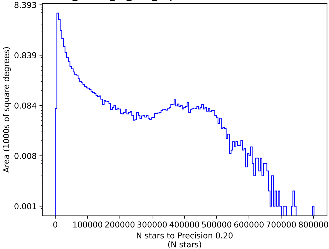
ddf_loaded_fl8_v3.4_10yrs i: N stars to Precision 0.20
