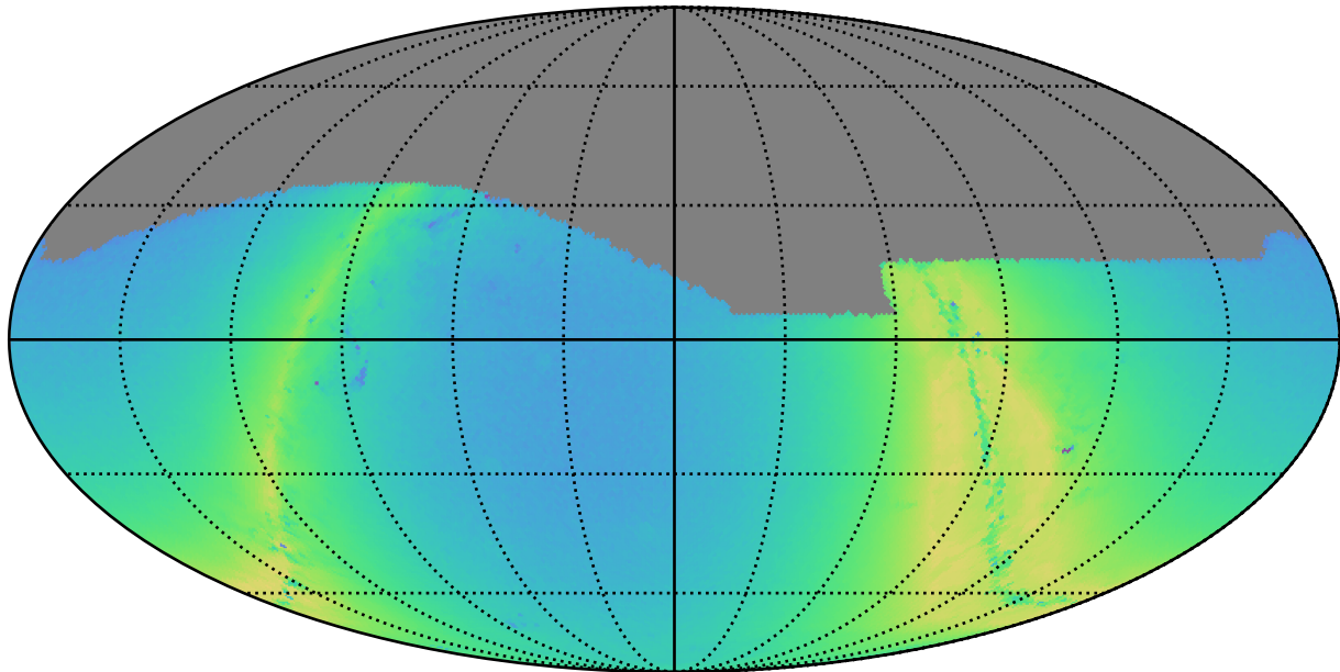
ddf_loaded_fl8_v3.4_10yrs g: N stars to Precision 0.20
