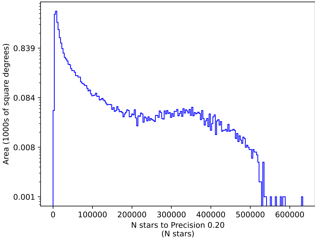
ddf_loaded_fl8_v3.4_10yrs g: N stars to Precision 0.20
