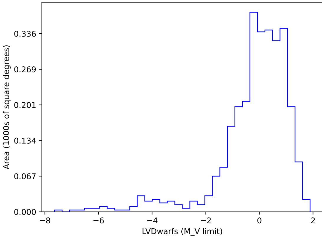
ddf_loaded_fl8_v3.4_10yrs gi SCP: LVDwarfs
