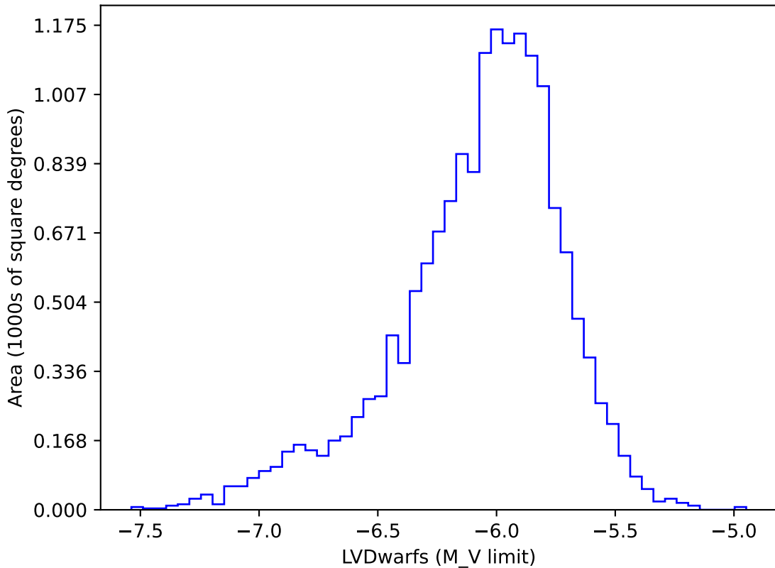
ddf_loaded_fl8_v3.4_10yrs gi: LVDwarfs
