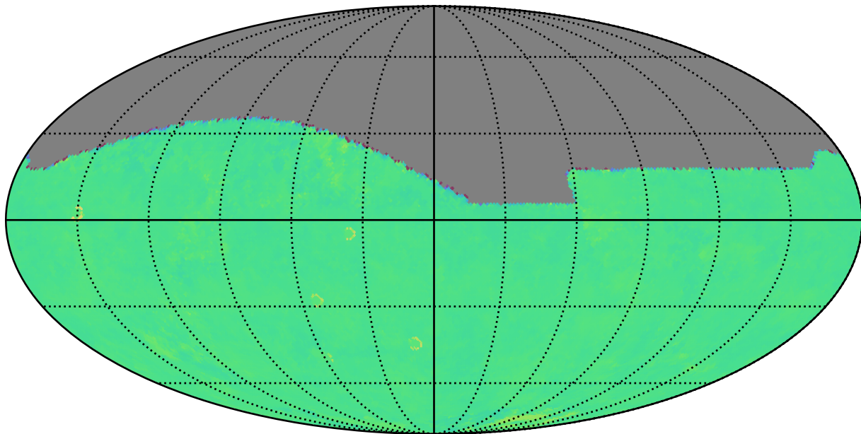
ddf_loaded_fl8_v3.4_10yrs z: Kuiper rotTelPos
