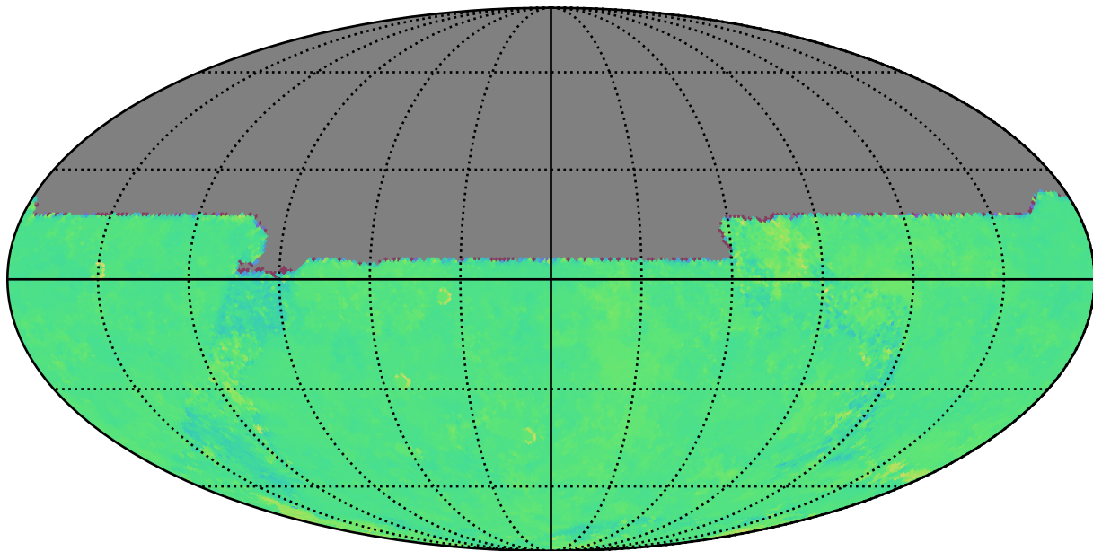
ddf_loaded_fl8_v3.4_10yrs u: Kuiper rotTelPos
