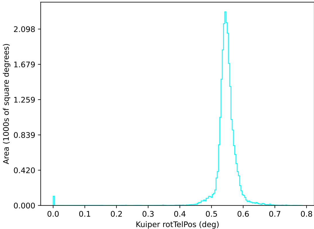
ddf_loaded_fl8_v3.4_10yrs u: Kuiper rotTelPos
