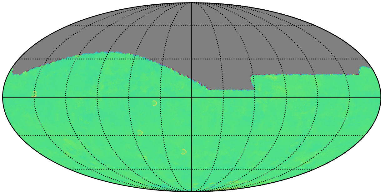
ddf_loaded_fl8_v3.4_10yrs r: Kuiper rotTelPos
