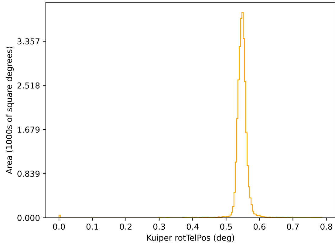
ddf_loaded_fl8_v3.4_10yrs r: Kuiper rotTelPos
