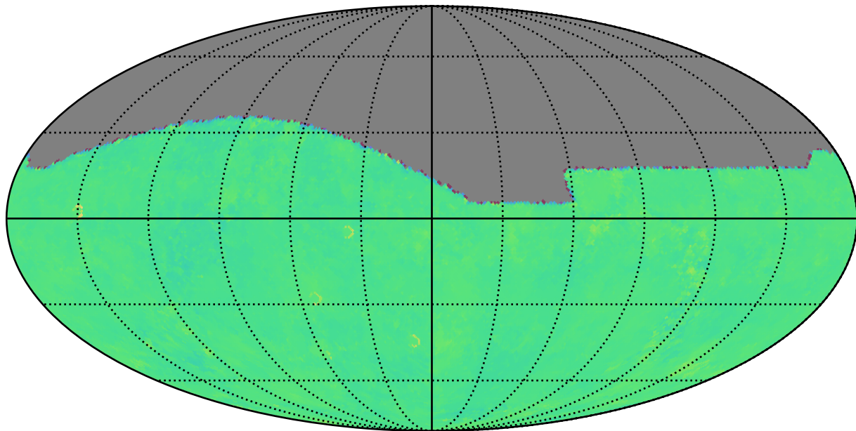
ddf_loaded_fl8_v3.4_10yrs g: Kuiper rotTelPos
