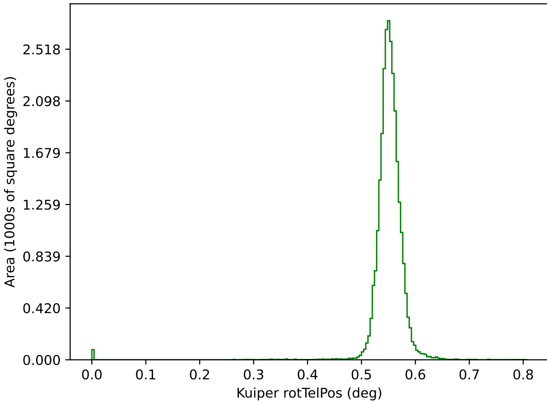
ddf_loaded_fl8_v3.4_10yrs g: Kuiper rotTelPos
