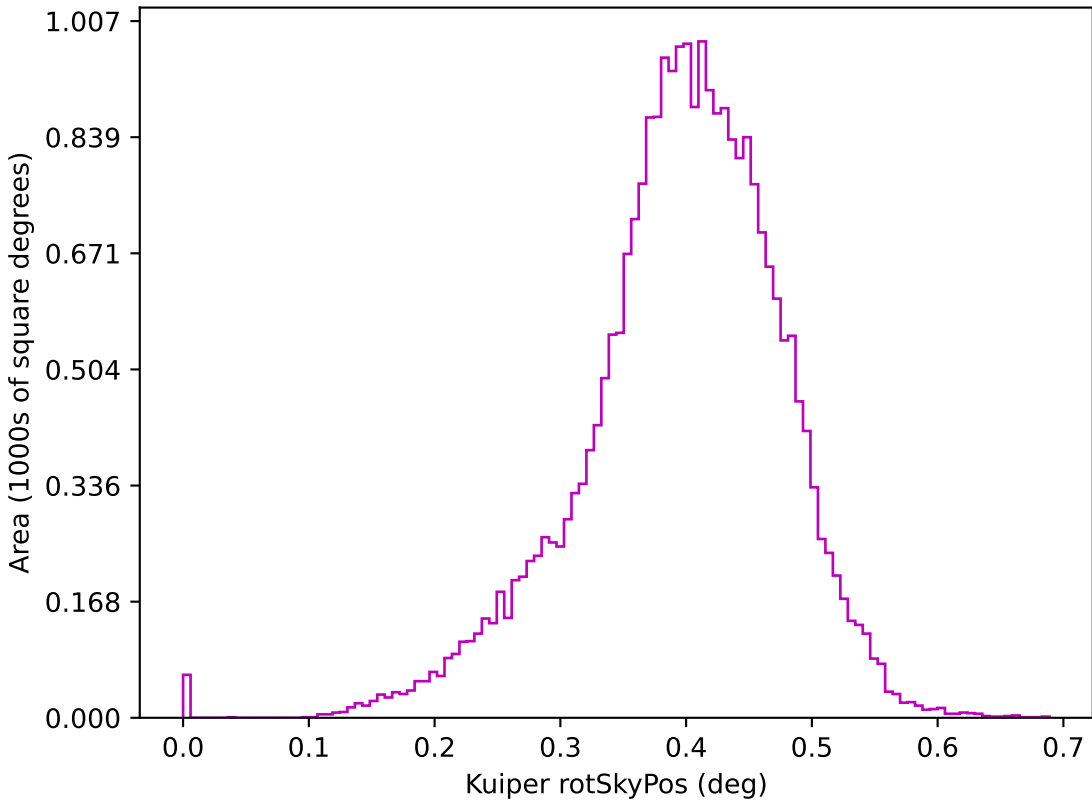
ddf_loaded_fl8_v3.4_10yrs z: Kuiper rotSkyPos
