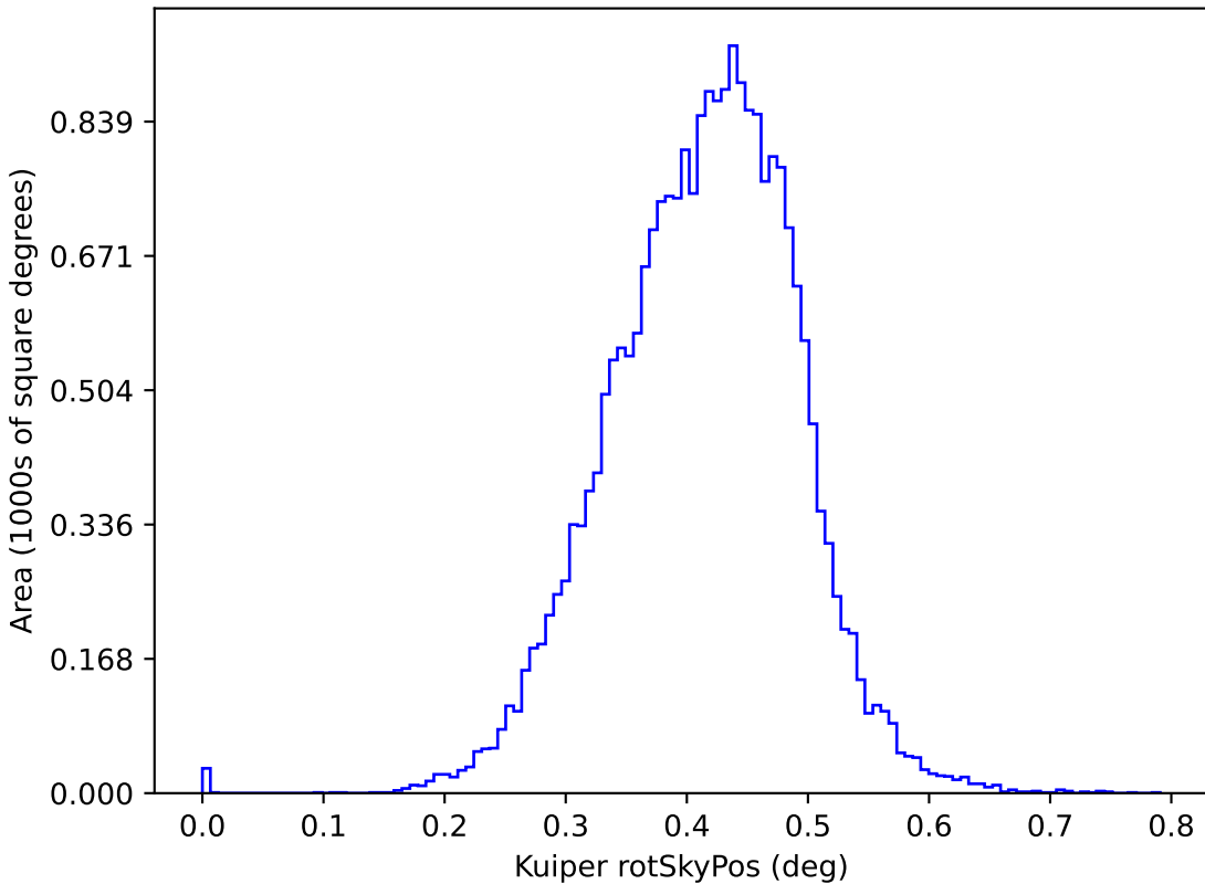
ddf_loaded_fl8_v3.4_10yrs y: Kuiper rotSkyPos
