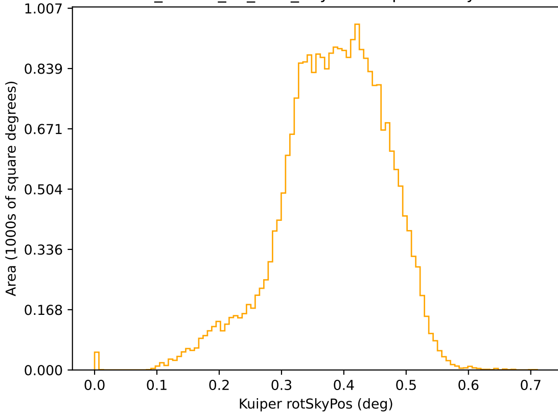
ddf_loaded_fl8_v3.4_10yrs r: Kuiper rotSkyPos
