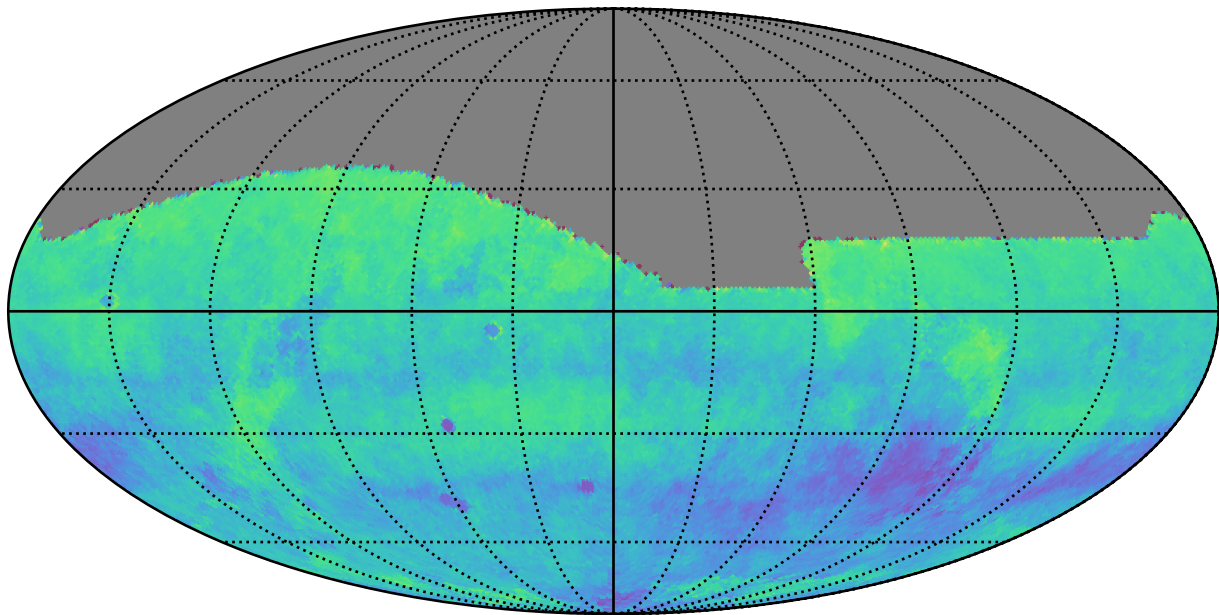
ddf_loaded_fl8_v3.4_10yrs i: Kuiper rotSkyPos
