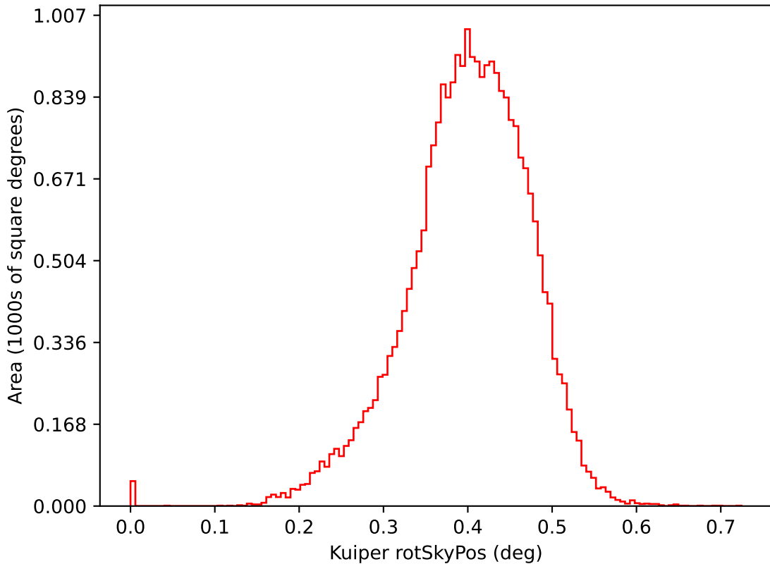
ddf_loaded_fl8_v3.4_10yrs i: Kuiper rotSkyPos
