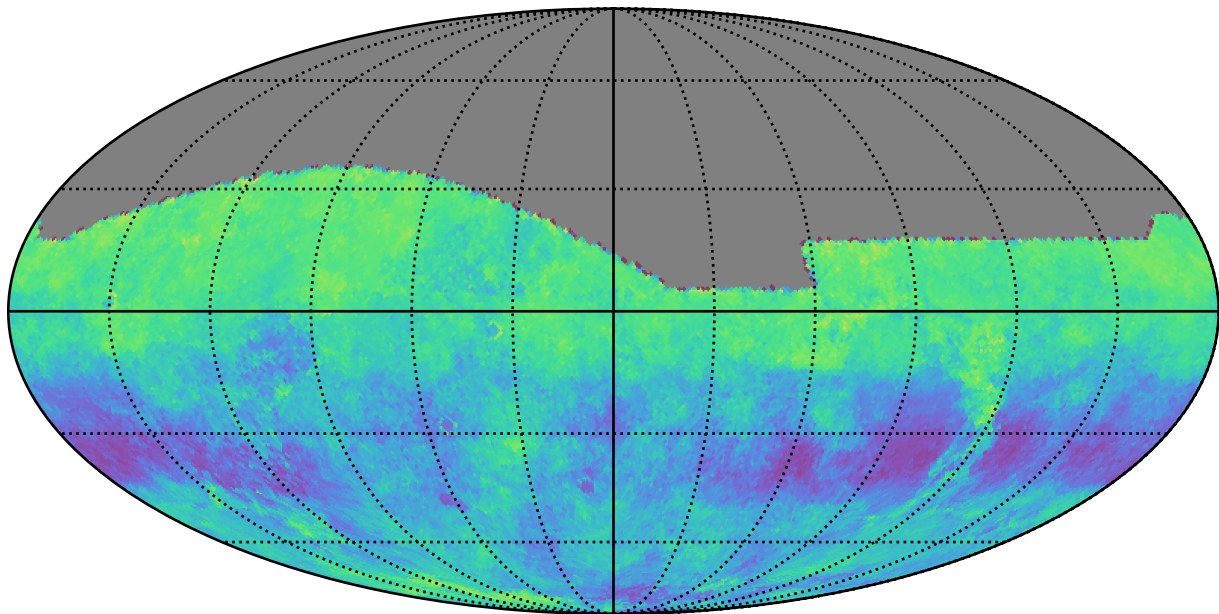
ddf_loaded_fl8_v3.4_10yrs g: Kuiper rotSkyPos
