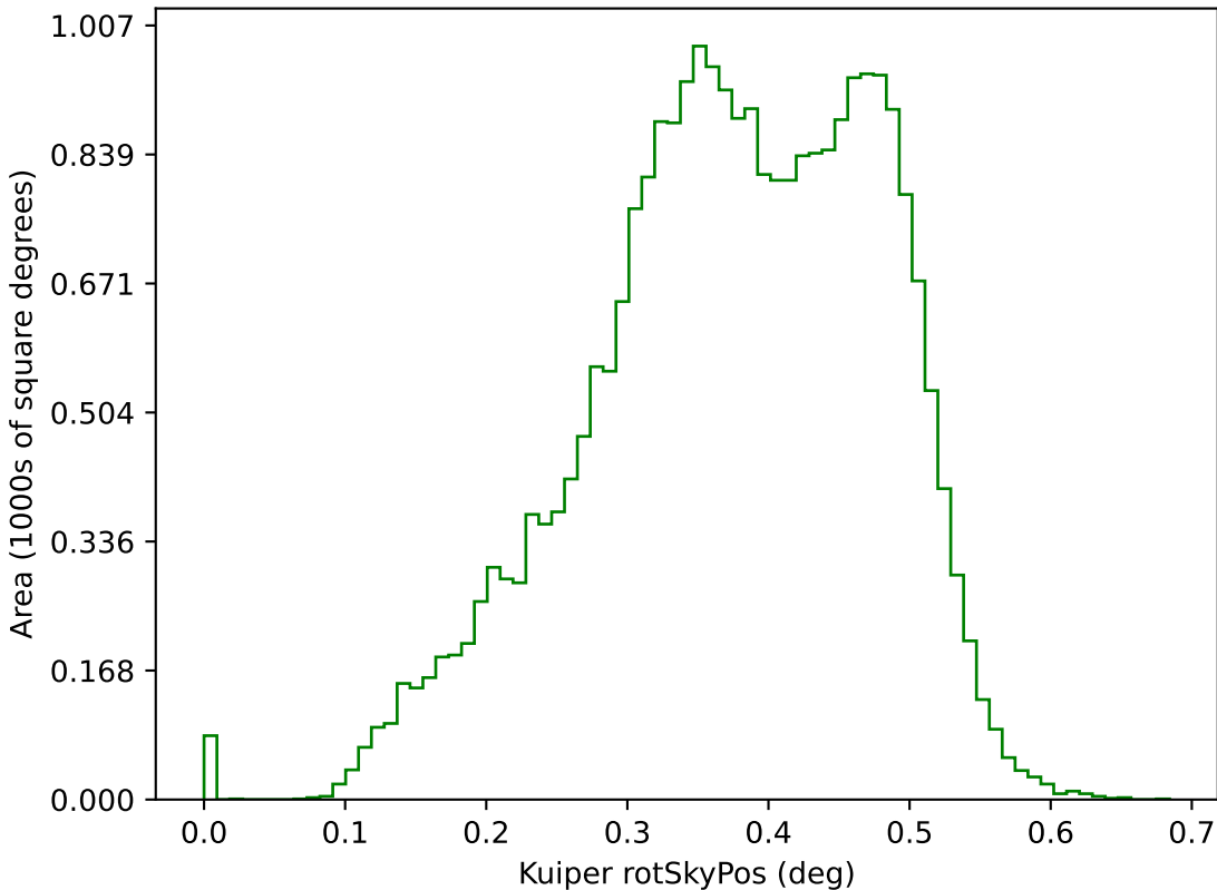
ddf_loaded_fl8_v3.4_10yrs g: Kuiper rotSkyPos
