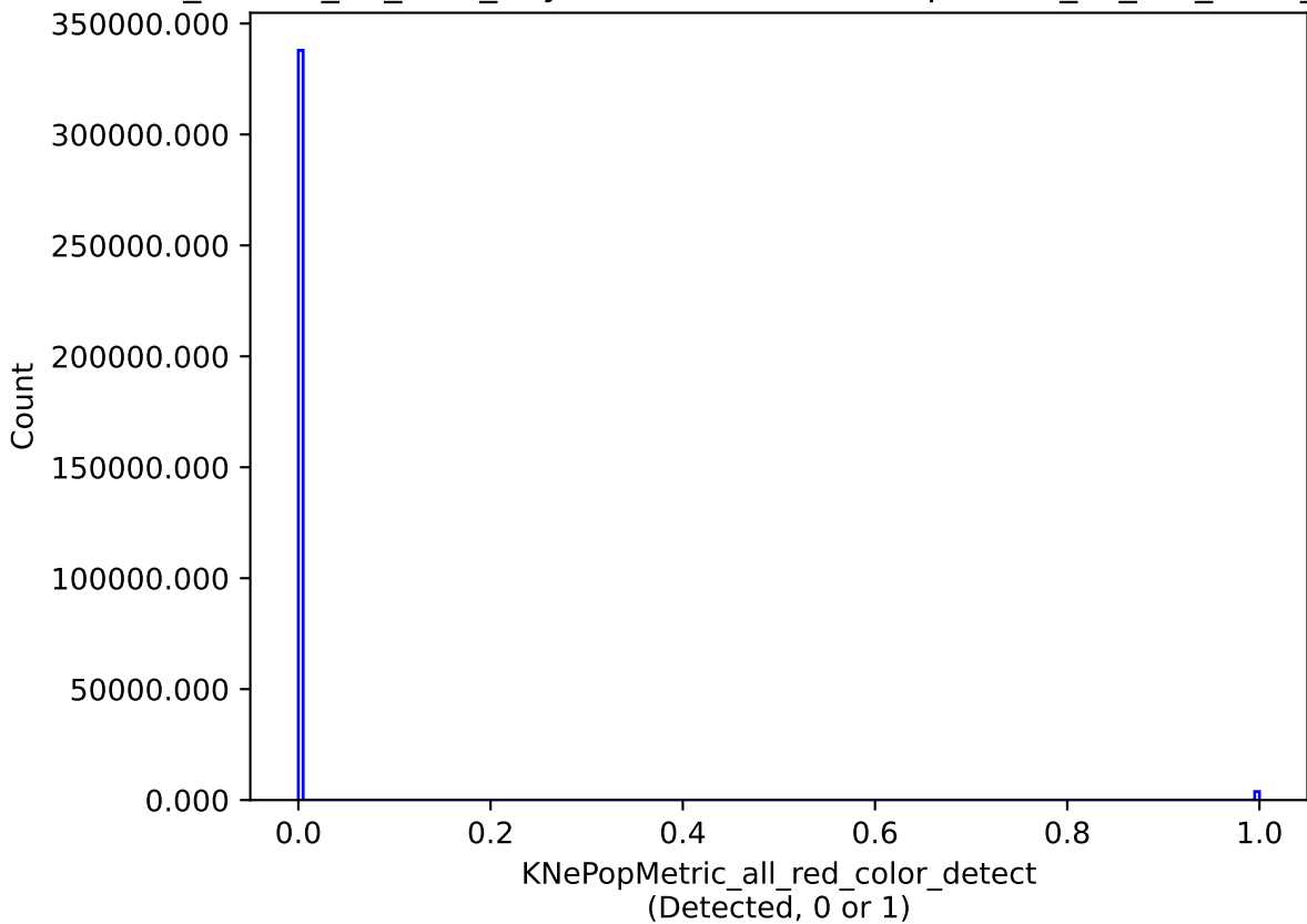
ddf_loaded_fl8_v3.4_10yrs all models: KNePopMetric_all_red_color_detect
