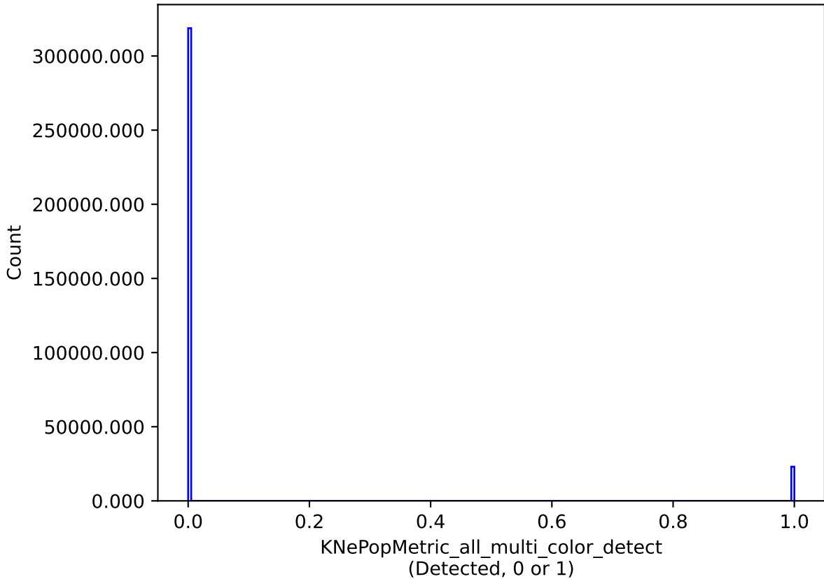
ddf_loaded_fl8_v3.4_10yrs all models: KNePopMetric_all_multi_color_detect
