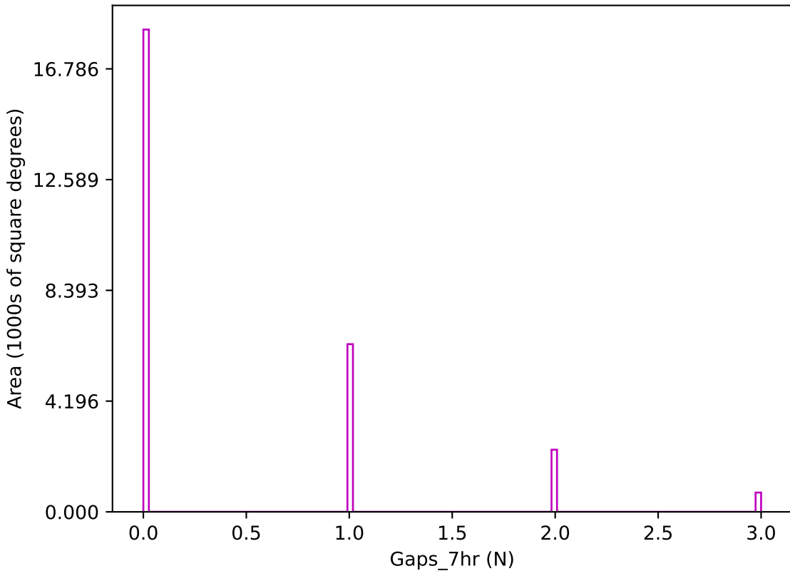
ddf_loaded_fl8_v3.4_10yrs z band: Gaps_7hr
